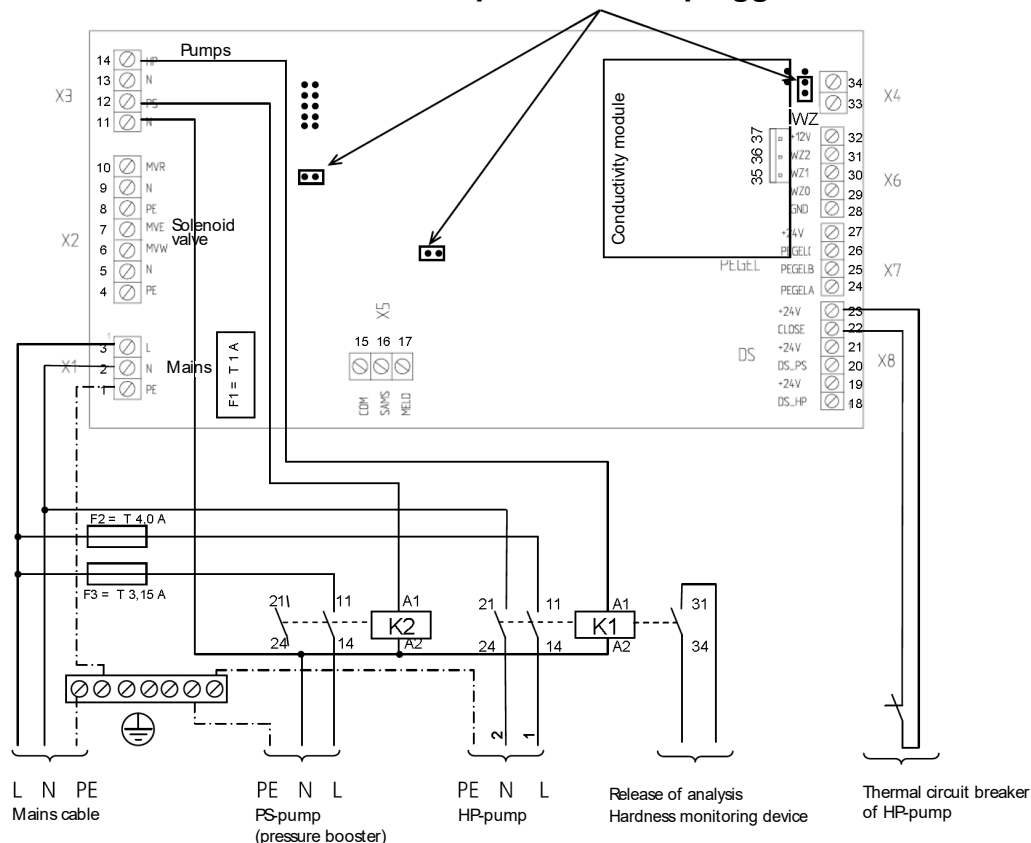
Fig. D-1: Printed circuit board assignment GENO-OSMO RO 125K
