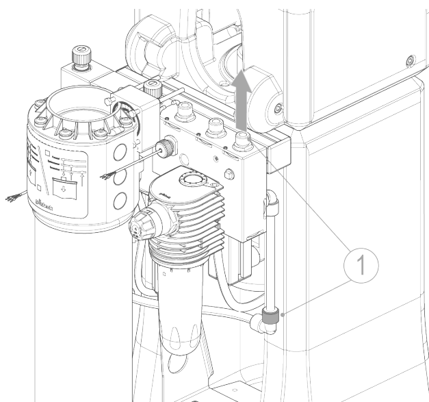
Fig. E-2: Permeate line RO 125K-TL
