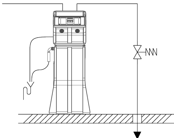
Fig. D-3: Withdrawal point below system level
