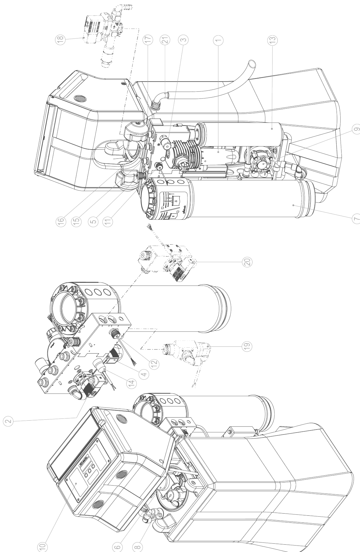
Fig. C-2: Exploded drawing of reverse osmosis system GENO-OSMO 125K-TS
