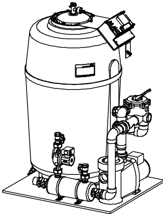
Fig. 1: Filter system GENO-mat® F 600 HK
