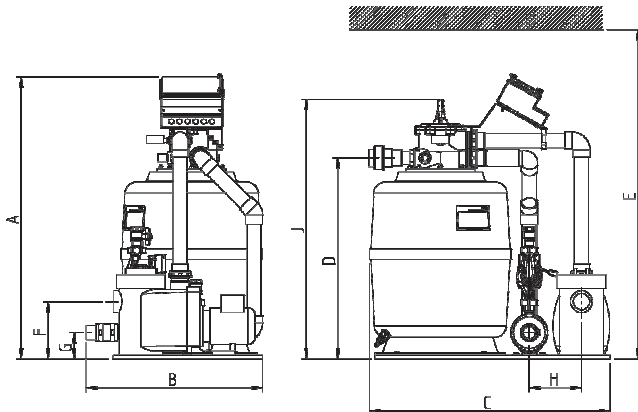
Fig. 2 Dimensional drawing of filter system GENO-mat® F 500 HK; AC
