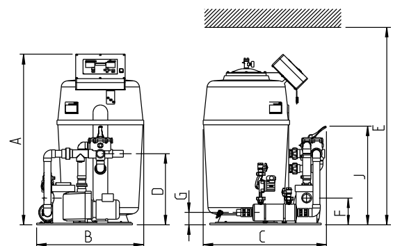
Fig. 3 Dimensional drawing of filter system GENO-mat® F 600 HK; RC
