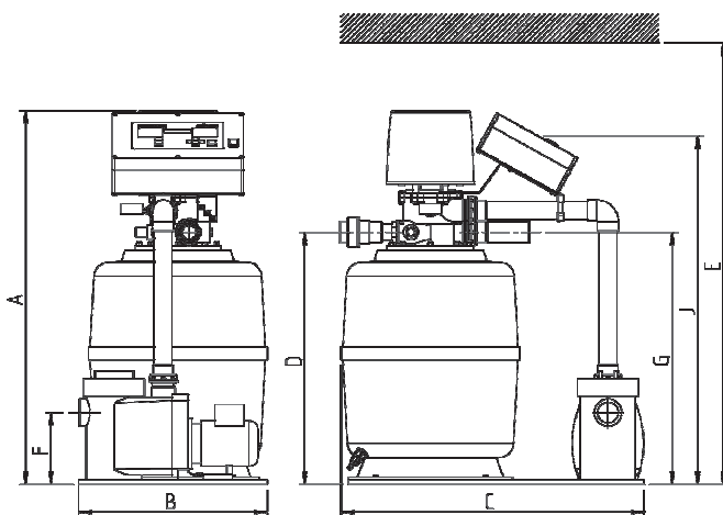
Fig. 2 Dimensional drawing of filter system GENO-mat® F 500 A
