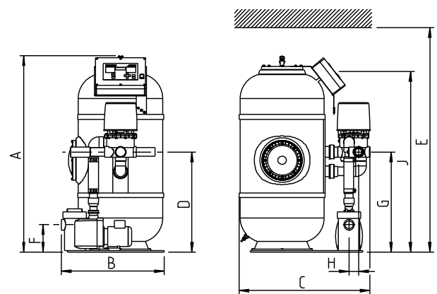
Fig. 3 Dimensional drawing of filter system GENO-mat® F 610 A
