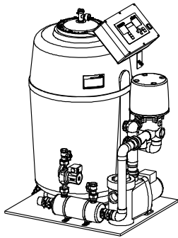
Fig. 1: Filter system GENO-mat® F 600 AK
