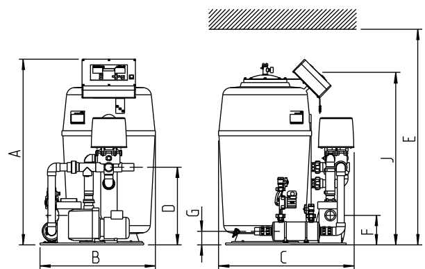
Fig. 3 Dimensional drawing of filter system GENO-mat® F 600 AK; RC
