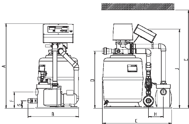
Fig. 2 Dimensional drawing of filter system GENO-mat® F 500 AK; RC
